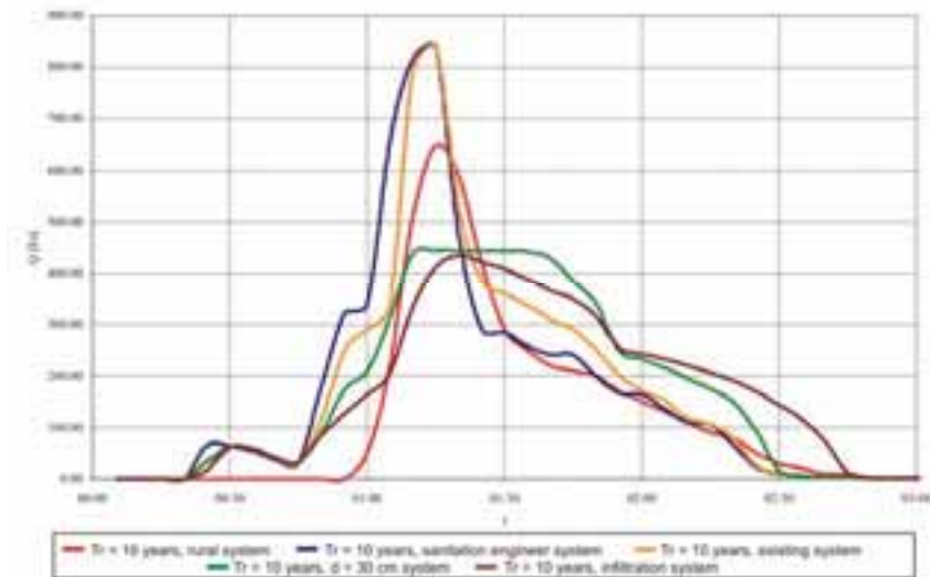
Figure 6.59. Output hydrographs for all the scenarios tested ( T_r = 10 years)
