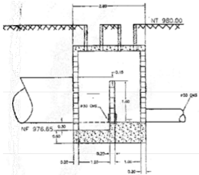
Figure 6.57. Detail of the construction of the storage and regulation chamber (Paso Fresco housing development, AMSS)
