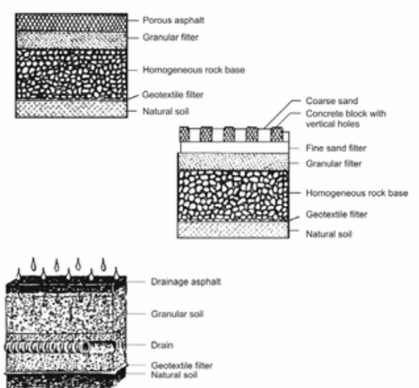
Figure 3.21. Pervious paving
