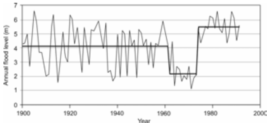
Figure 2.4. Maximum annual levels of the river Paraguay at Ladário and mean for the periods: (a) 1900-1961; (b) 1961-1973; (c) 1973-1991
