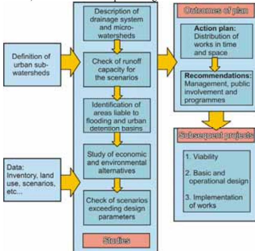
Figure 5.2. Structural measures
