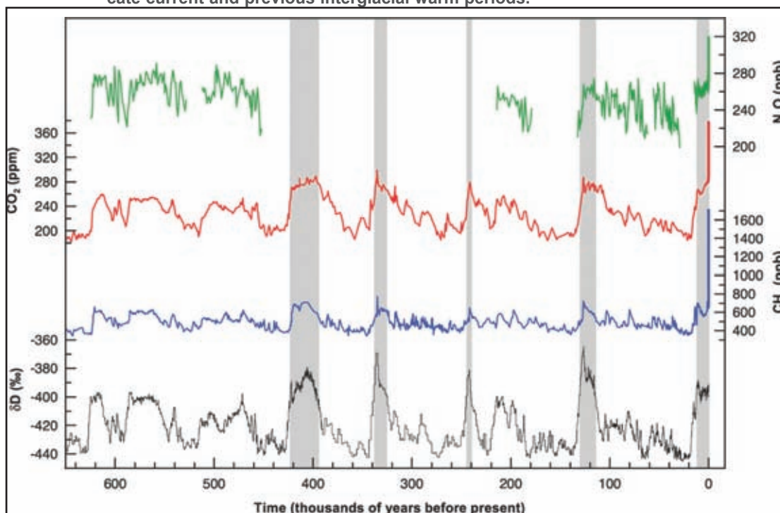
Figure 2.3: Variations of deuterium ( \delta\text{D} ) in Antarctic ice, and of carbon dioxide ( \text{CO}_2 ), methane ( \text{CH}_4 ) and nitrous oxide ( \text{N}_2\text{O} ) in air trapped within ice cores. Shaded bands indicate current and previous interglacial warm periods.
