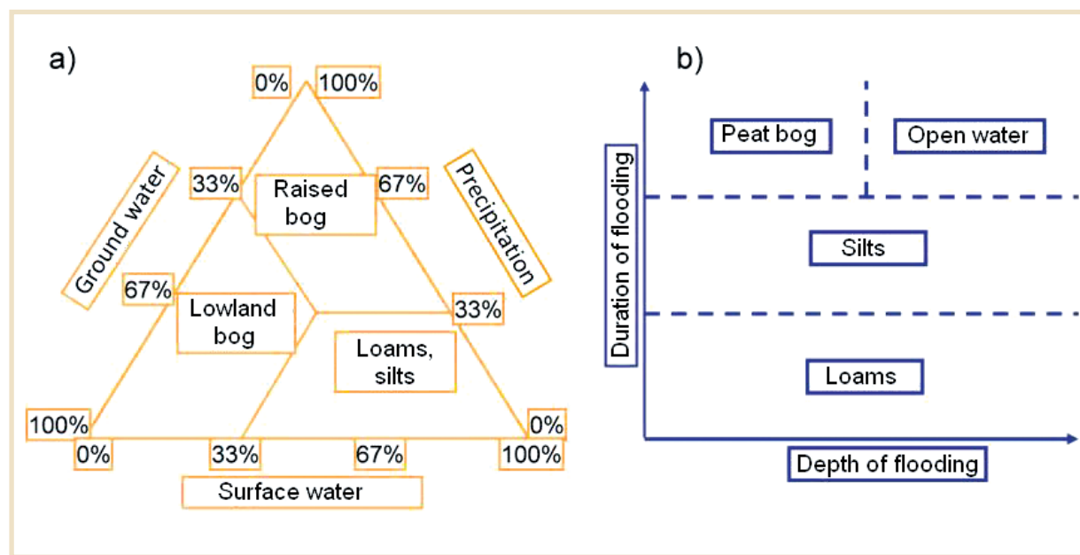
Figure 7. The relationship between different kinds of water alimenting the wetland, and type of wetland: a) kind of water, b) duration and water level during flood. Source: Okruszko, 2005
