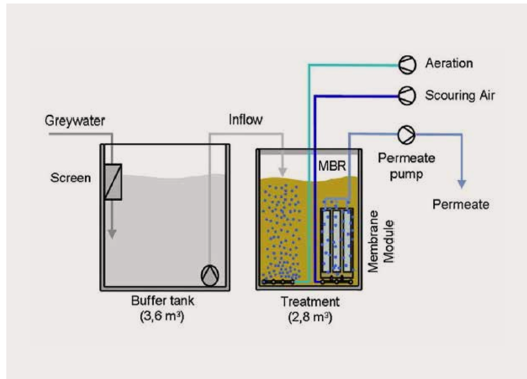
Fig.11: Above: Scheme of greywater recycling system with MBR technology (source: Catalogue of Technologies for Integrated Urban Water Management , 2014) Left: Greywater recycling plant with MBR technology, in Malta (source: SYSTEMA AZUD, S.A.)
