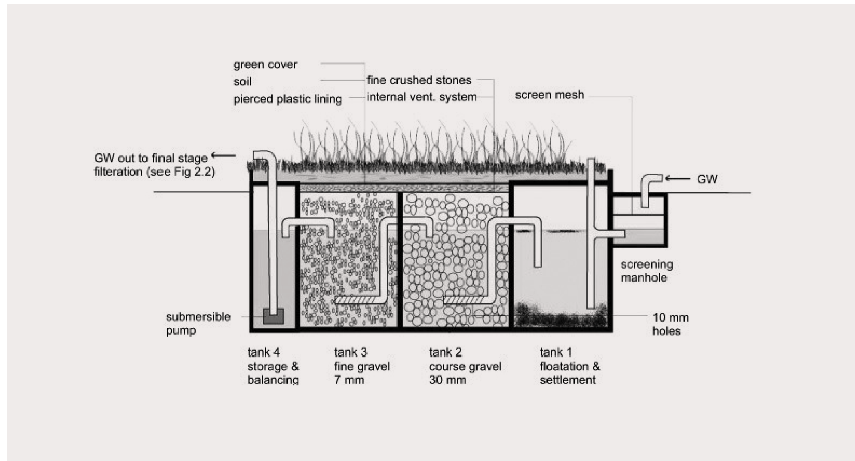
Fig.9: Physical greywater recycling system (Original source: Physical greywater treatment system used in Qebia Village, Palestine (Source: Burnat and Eshtayah, 2010)
